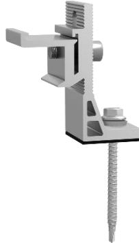
Tin Interface A with ezClick connection for ECO-Rail Part Number: ER-I-05A/EZC/ECO (barcode: 10-001-00177)
