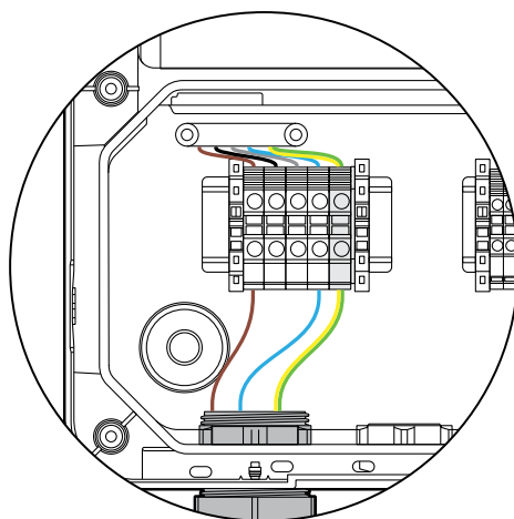
Figure 1: Wiring diagram of single-phase with Neutral
