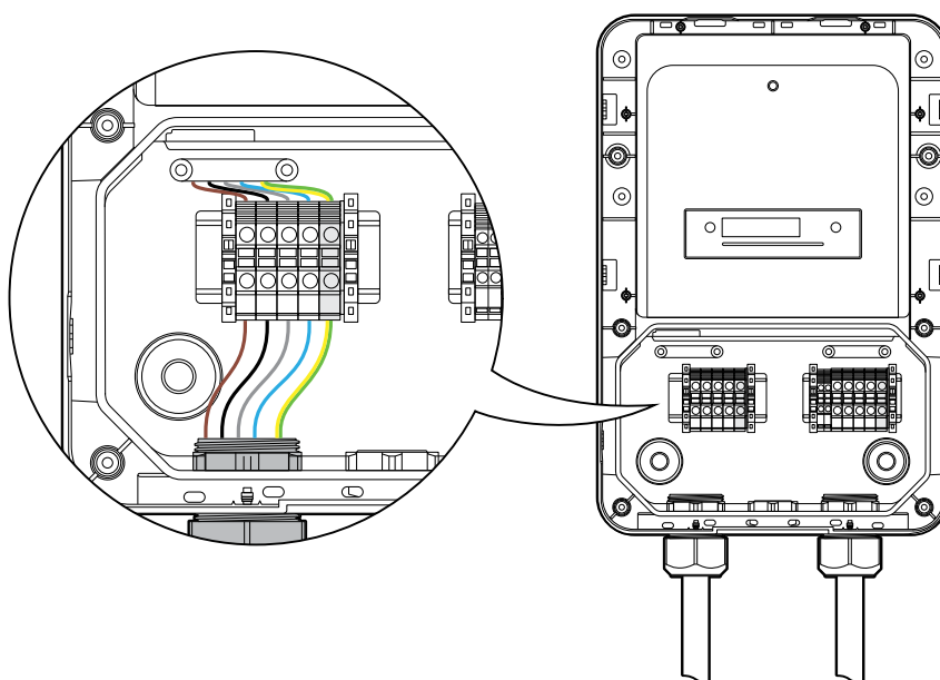
Figure 2: Wiring diagram of three-phase with Neutral
