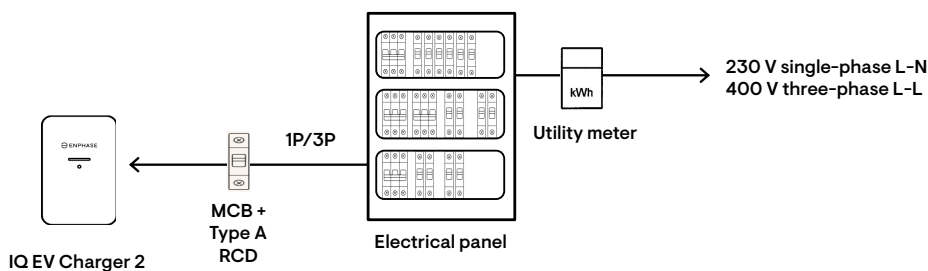
Figure 1: Standalone configuration
