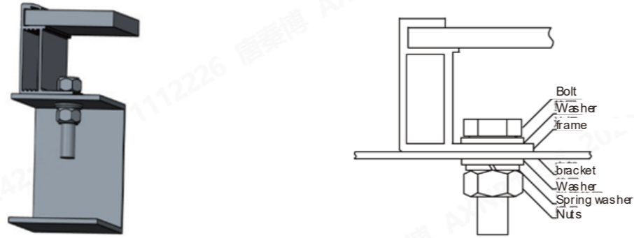
Module Mounting Holes
