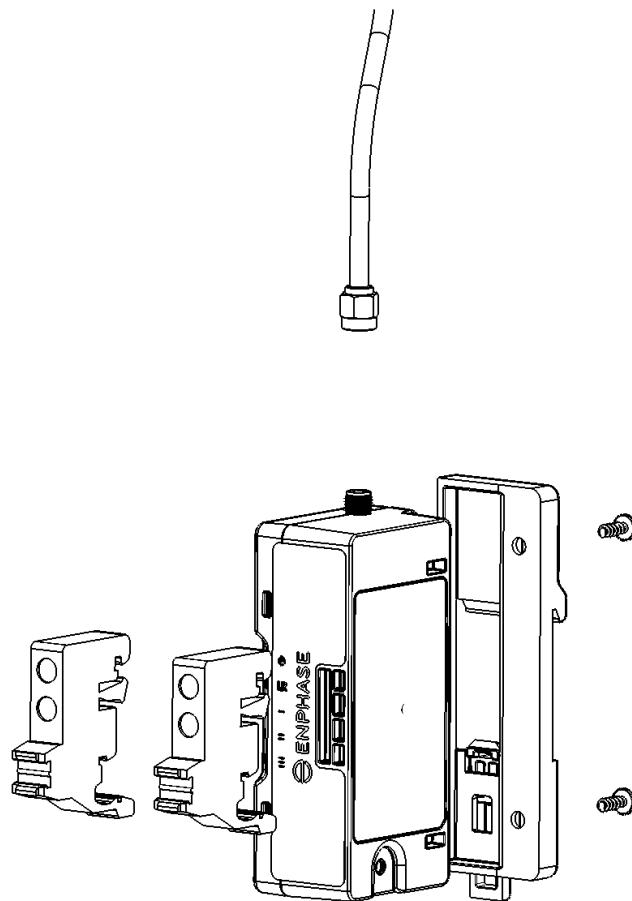
Figure 1: Installing the external antenna to CELLMODEM-07
