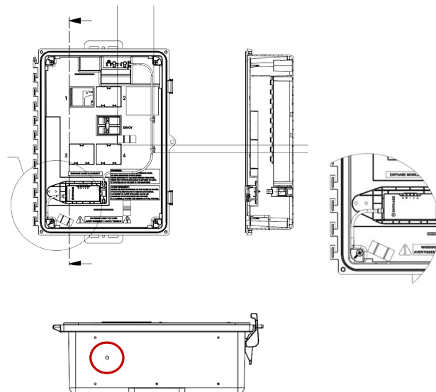
Figure 3: Custom external conduit point to route the cable
