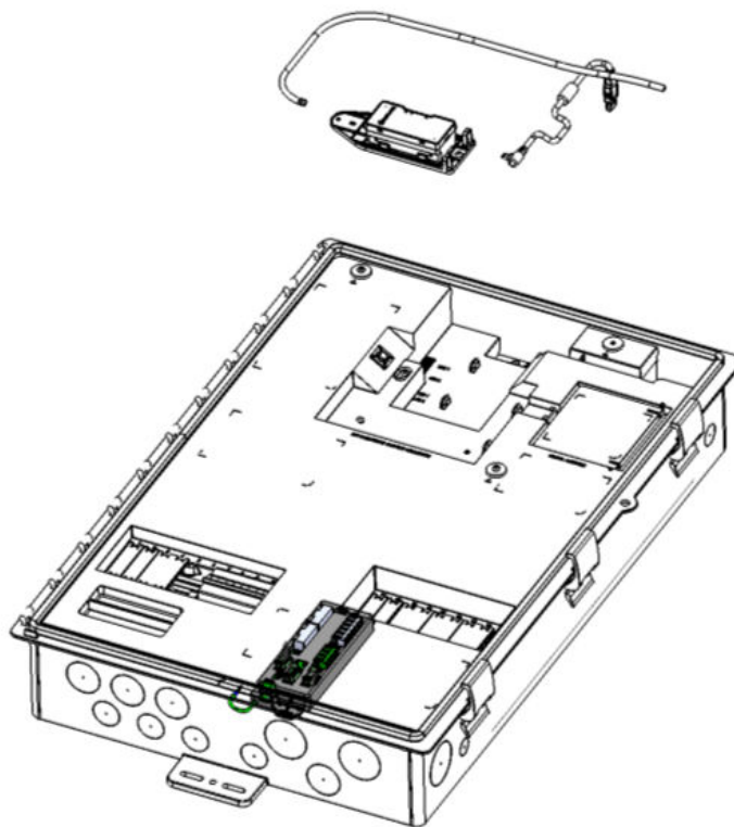
Figure 5: Placing the CELLMODEM-07 with external antenna into IQ System Controller 3 INT
