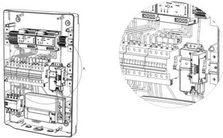
Figure 4: Placing the CELLMODEM-07 with external antenna into IQ Combiner EU
